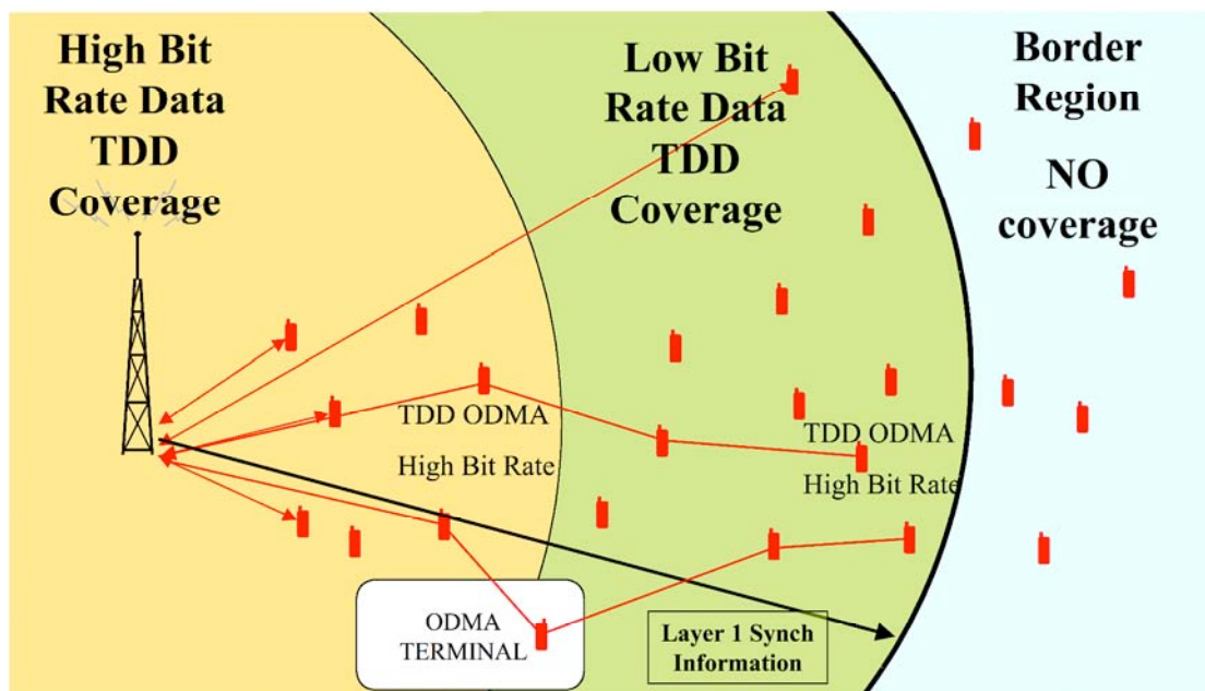
Figure 1: ODMA Border Coverage
