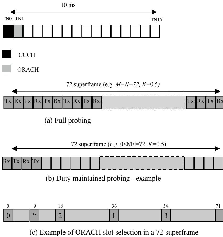
Figure 4: ORACH Superframe selection
