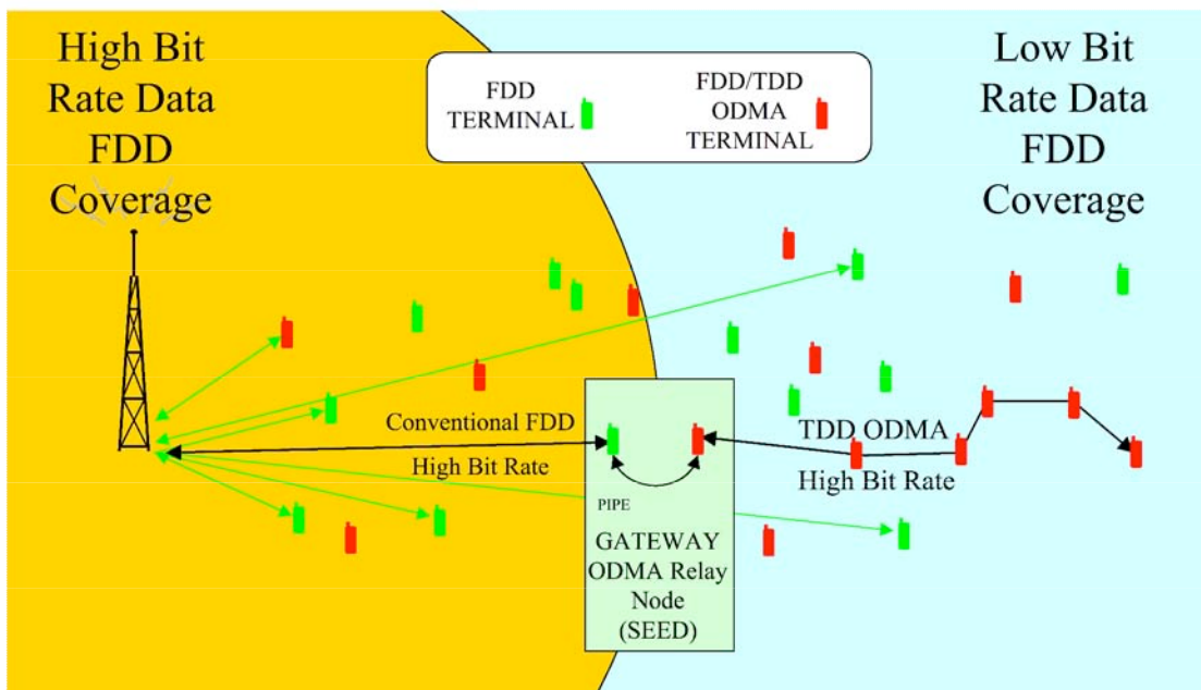
Figure 3: ODMA concept diagram with last hop
